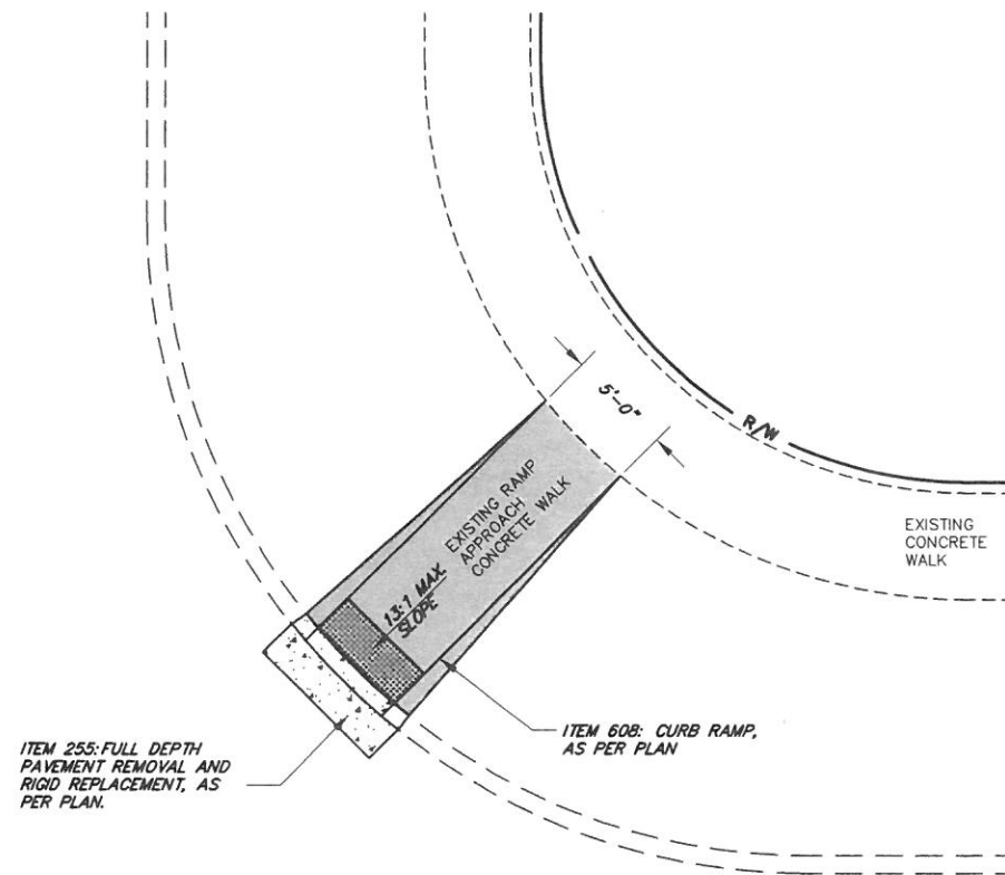
TYPE A1 CURB RAMP REPLACEMENT PLAN
