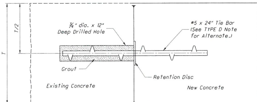
TYPE D (DRILLED TIED LONGITUDINAL) JOINT
