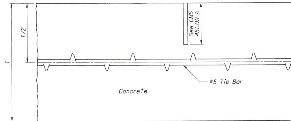
SAWED JOINT
