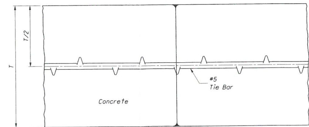
BUTT JOINT w/ TIE BAR
