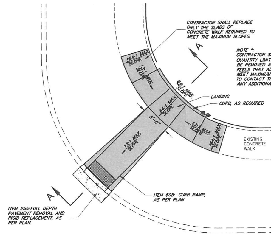
TYPE A2 CURB RAMP, APPROACH WALK & LANDING REPLACEMENT PLAN
