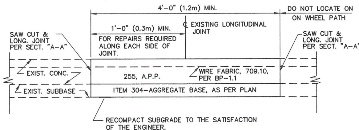
SECTION "F-F" LONGITUDINAL JOINT REPAIR
